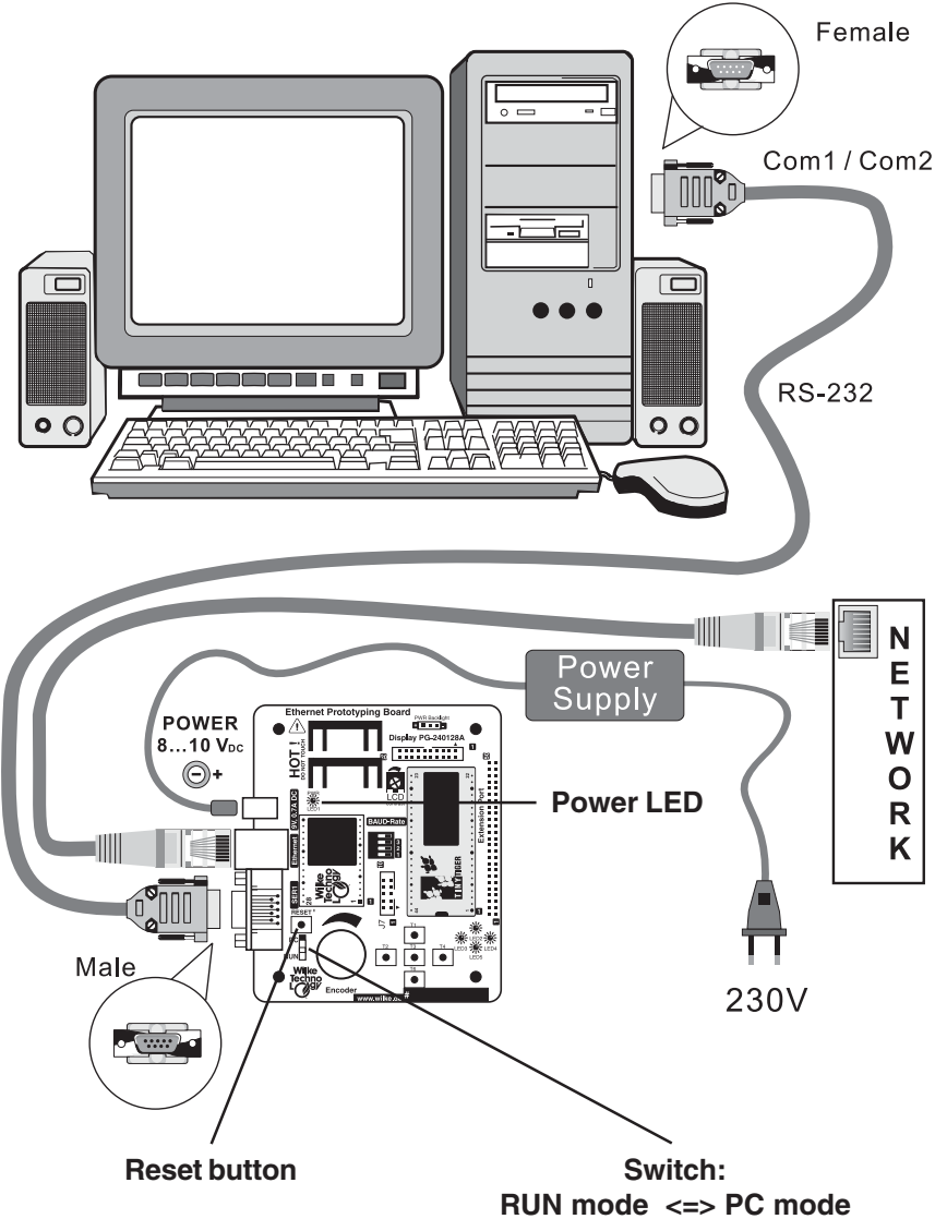
Fig. 1: Connections for Ethernet Starter Kit I
